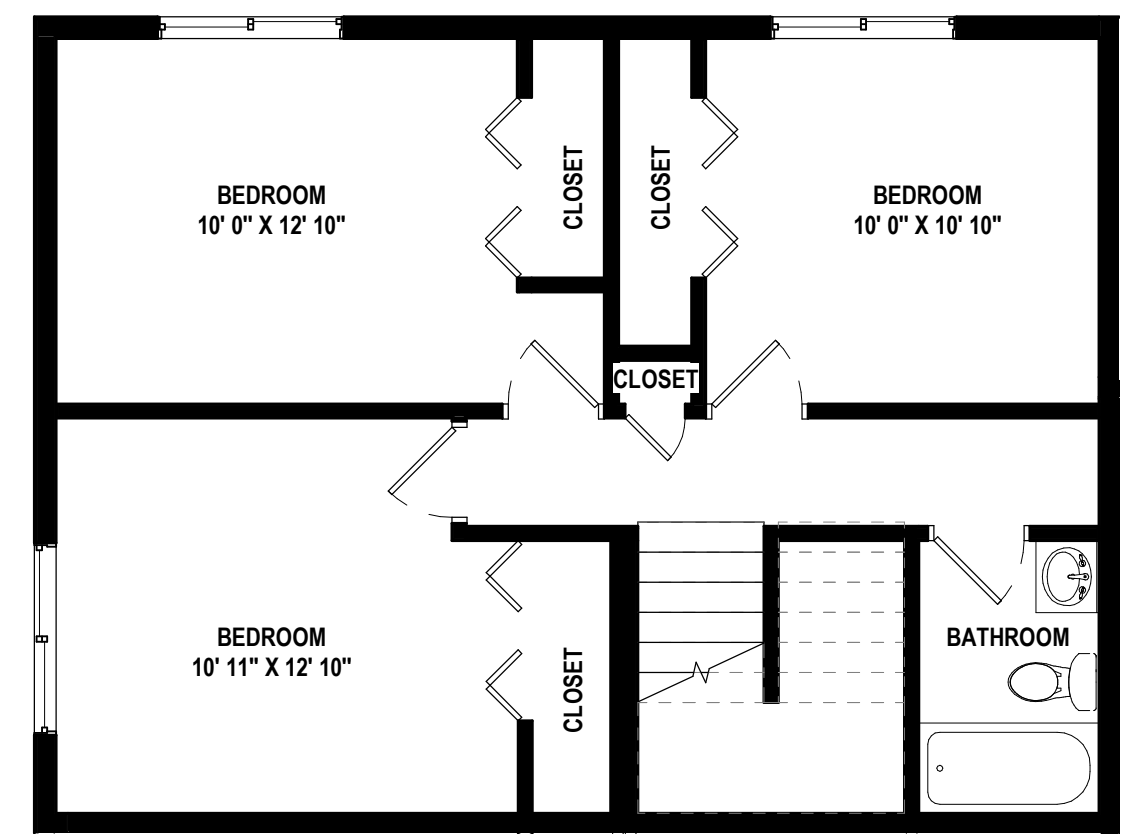
③ Marketing Townhouse Level 2 3/16" = 1'-0"
